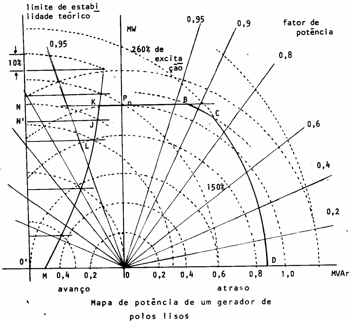
FIGURE 6.22 Complex power locus per phase.
