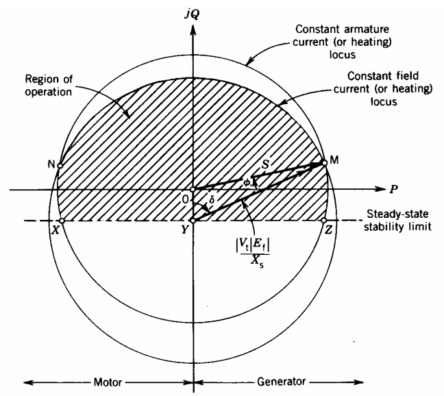
FIGURE 6.23 Capability curves of a synchronous machine.
